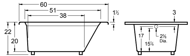
All bathtub dimensions are ± 1/2".
