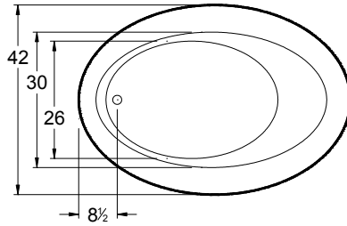
Tub pictured with optional waste & overflow.
