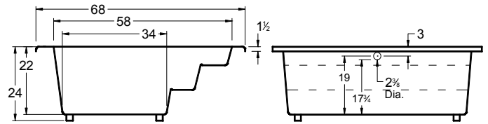
All bathtub dimensions are ± 1/2"
